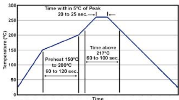
Time/Temperature Soldering Profile
