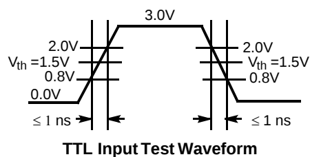
Figure 9. Test Loads and Waveforms
