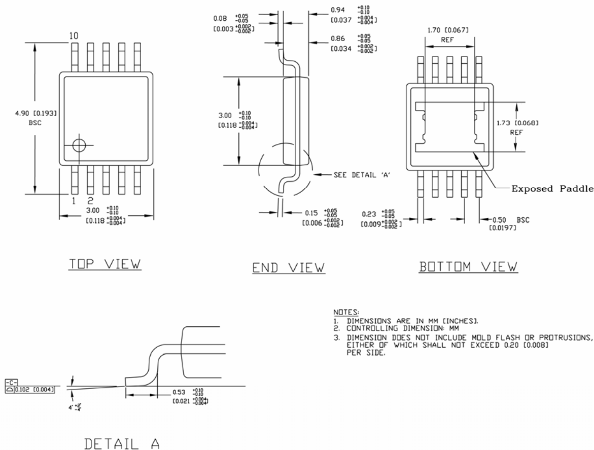
10-Lead e-PAD MSOP (MME)
