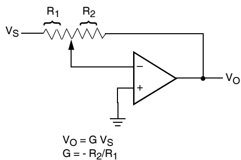
Inverting Amplifier
