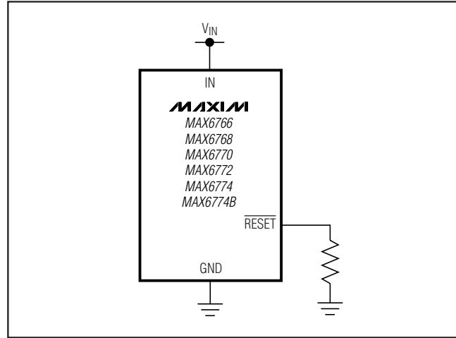
Figure 5. Ensuring RESET Valid to V_{IN} = 0V
