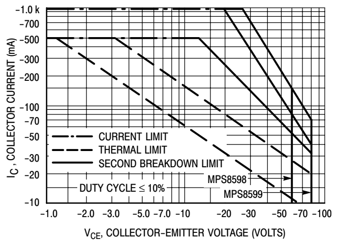
Figure 10. MPS8598/99 Active-Region Safe Operating Area
