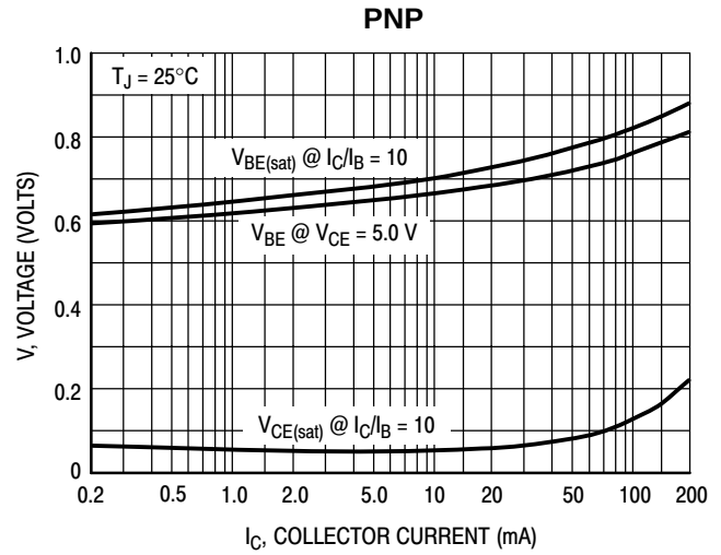
Figure 14. MPS8598/99 "ON" Voltages
