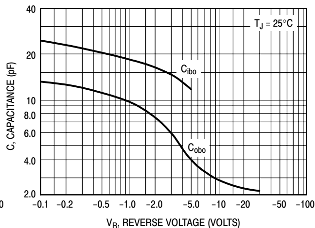
Figure 6. MPS8598/99 Capacitance
