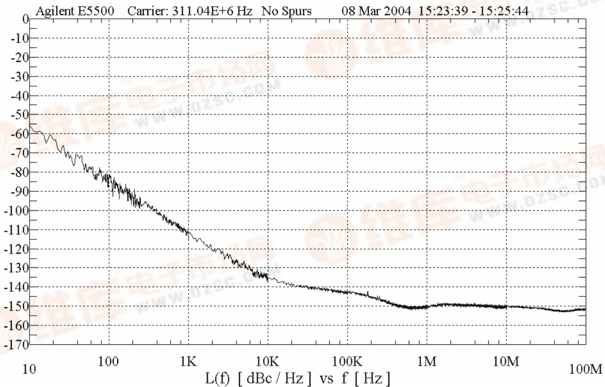
Figure 1: 2x AFM Phase Noise at 311.04MHz
