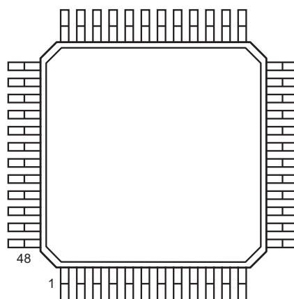
48-Lead LQFP (FG) (7x7x1.4mm) (top view)
