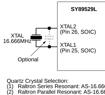
Figure 1. Crystal Interface
