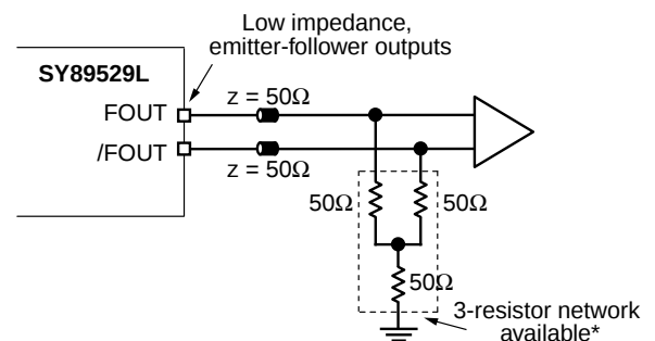
Figure7. LVPECL Output Termination
