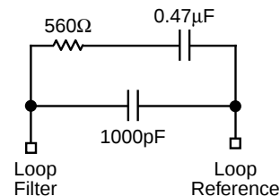
Figure 2. External Loop Filter Connection
