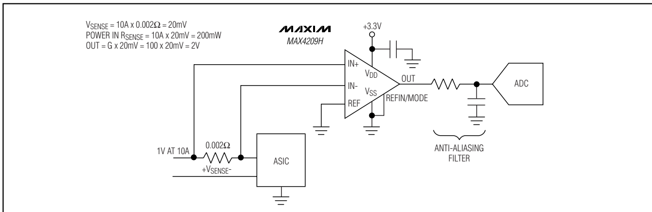
Figure 5. MAX4208/MAX4209 Used as Precision Current-Sense Amplifiers for Notebook Computers with V_{SENSE} of 20mV
