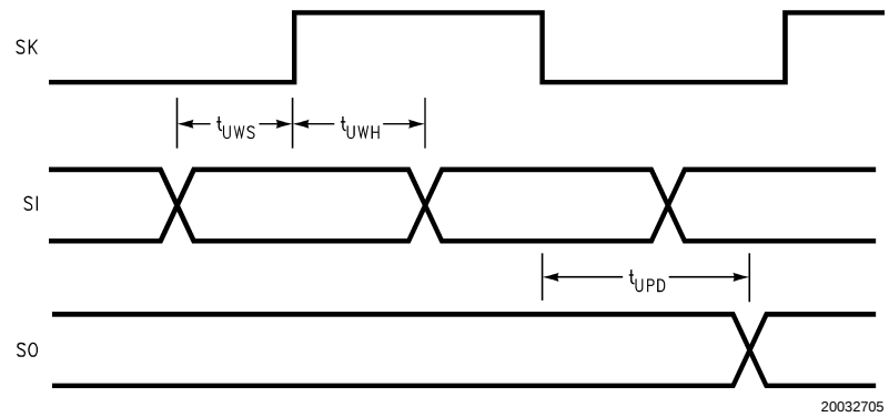
FIGURE 1. MICROWIRE/PLUS Timing
