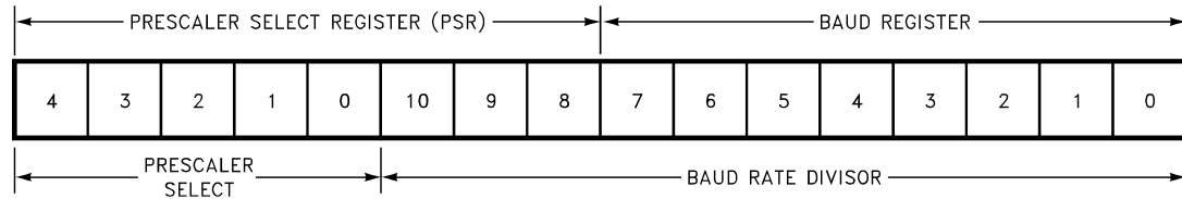
FIGURE 25. USART BAUD Clock Divisor Registers
