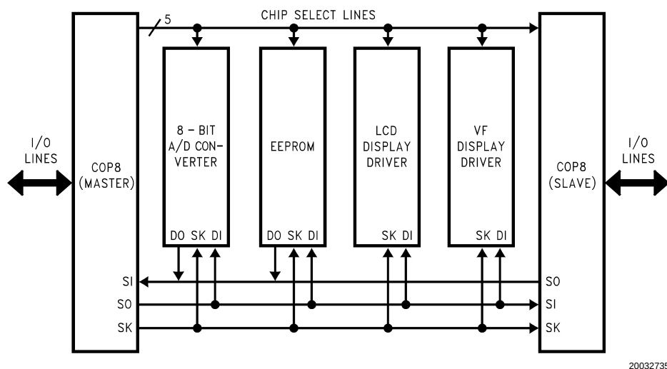
FIGURE 29. MICROWIRE/PLUS Application
