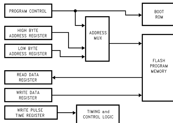
FIGURE 13. Block Diagram of ISP
