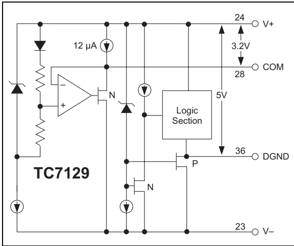
Figure 4-15: Digital Ground (DGND) and Common Outputs.
