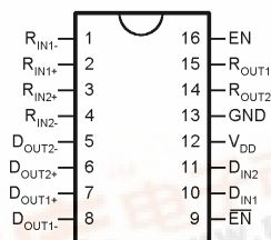
Dual-In-Line
