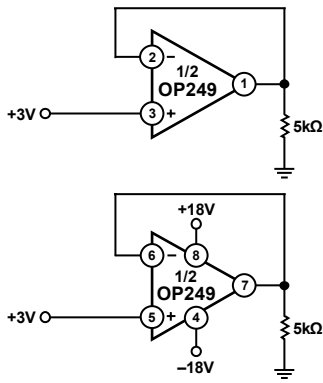
Figure 40. Burn-In Circuit
