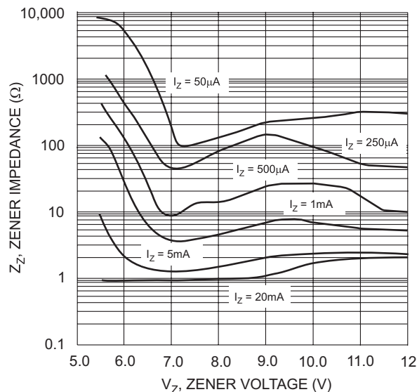
Fig. 10 Typical Zener Impedance Characteristics, DDZ5V6BS - DDZ12CS
