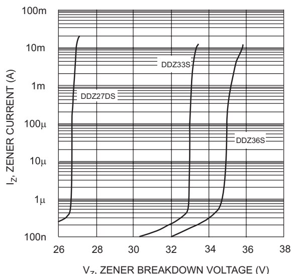
Fig. 8 Typical Reverse Characteristics, DDZ27DS - DDZ36S
