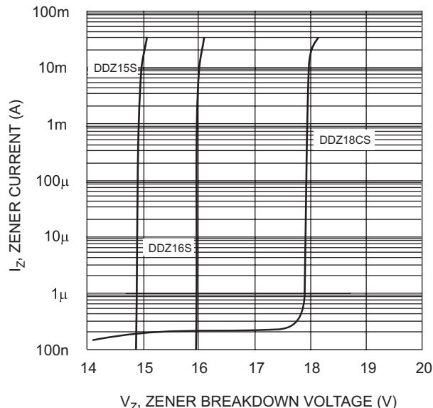
Fig. 6 Typical Reverse Characteristics, DDZ15S - DDZ18CS
