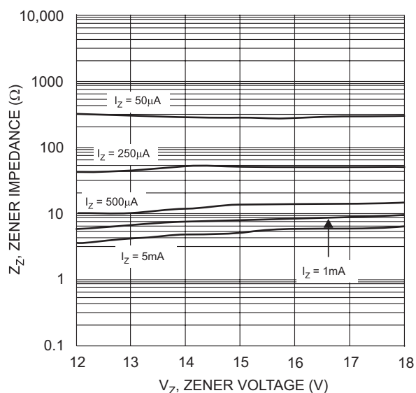
Fig. 11 Typical Zener Impedance Characteristics, DDZ12CS - DDZ18CS
