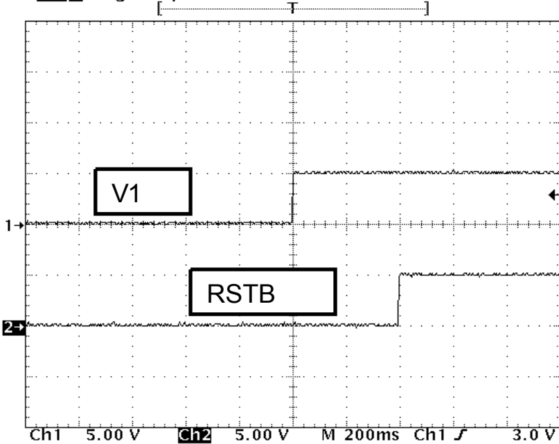
RESETB Timeout Period (400mS)
