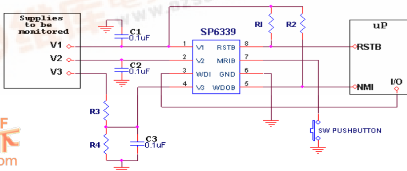
Configured for using Open-Drain outputs
