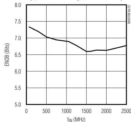
ENOB vs. ANALOG INPUT FREQUENCY ( f_{CLK} = 2.49856Gsp/s , A_{IN} = -1dBFS )
