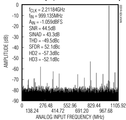
FFT PLOT (16,384-POINT DATA RECORD)
