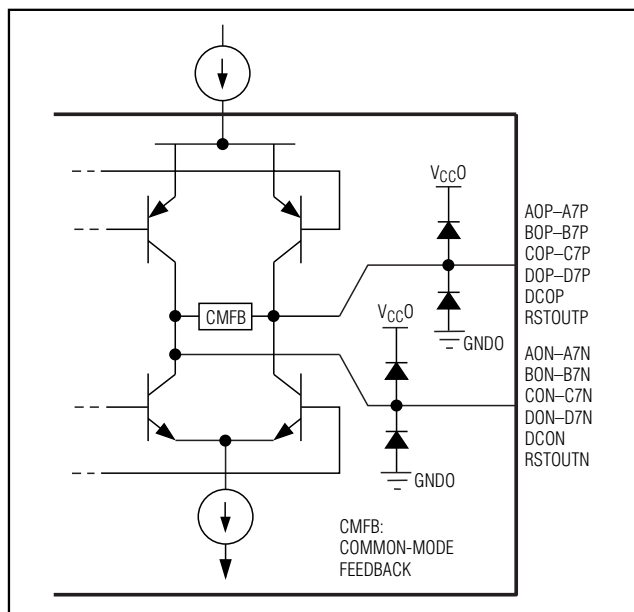
Figure 5. Simplified LVDS Output Circuitry
