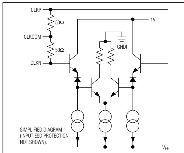
Figure 12. Clock Input Structure
