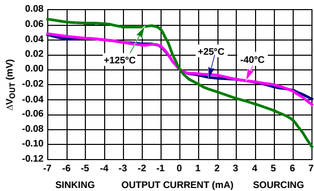
FIGURE 6. LOAD REGULATION
