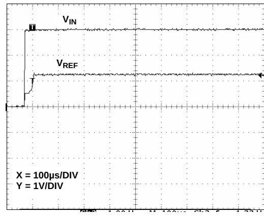
FIGURE 11. TURN-ON TIME
