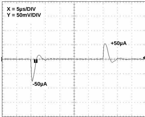
FIGURE 14. LOAD TRANSIENT RESPONSE
