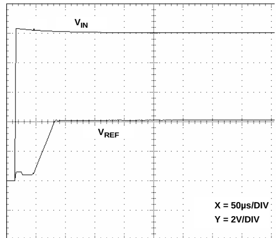
FIGURE 39. TURN-ON TIME
