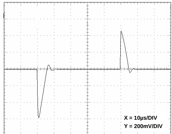
FIGURE 37. LINE TRANSIENT RESPONSE, NO CAPACITIVE LOAD
