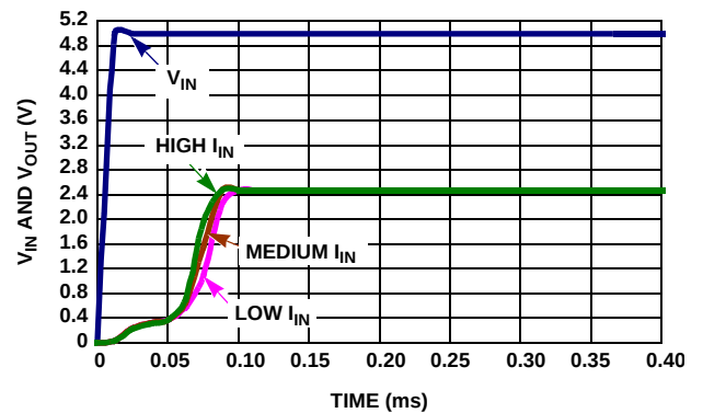
FIGURE 25. TURN-ON TIME
