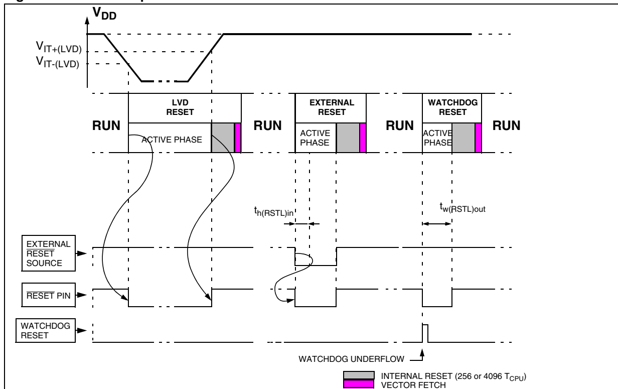
Figure 17. RESET Sequences
