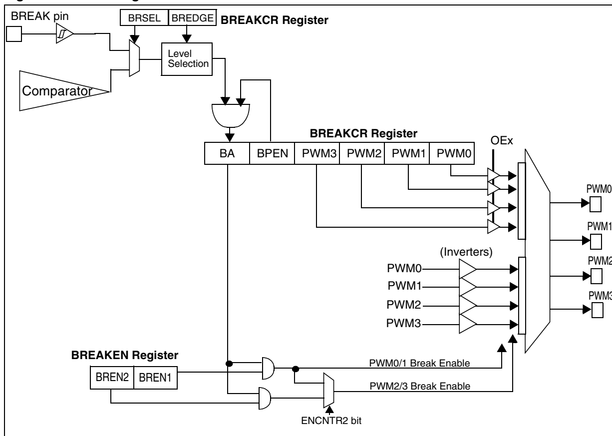
Figure 41. Block Diagram of Break Function
