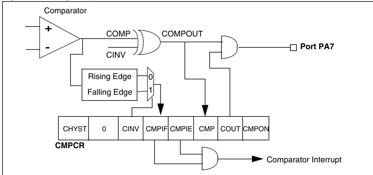
Figure 62. Analog Comparator
