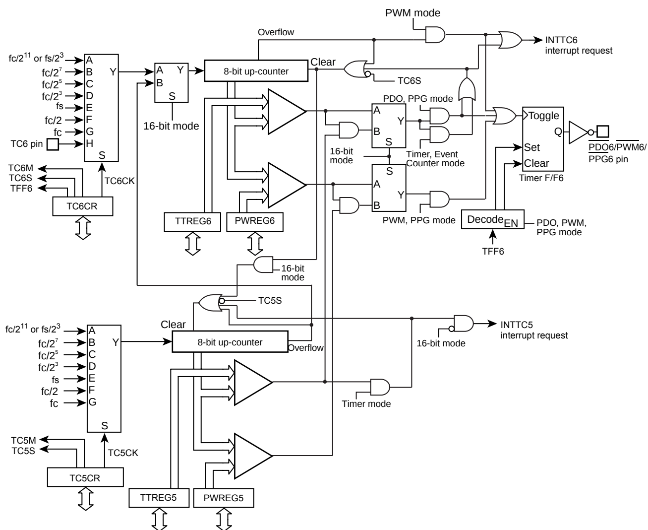
Figure 10-1 8-Bit TimerCounter 5, 6
