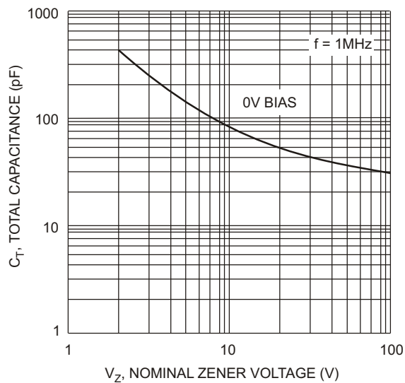
Fig. 2 Typical Capacitance
