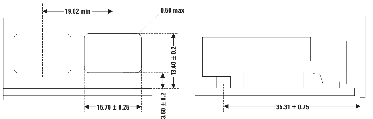
Figure 18. Host Frontplate Layout (dimensions in mm)
