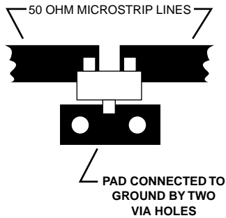
Figure 33. Circuit Layout.
