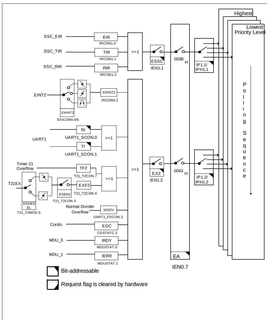
Figure 16 Interrupt Request Sources (Part 3)
