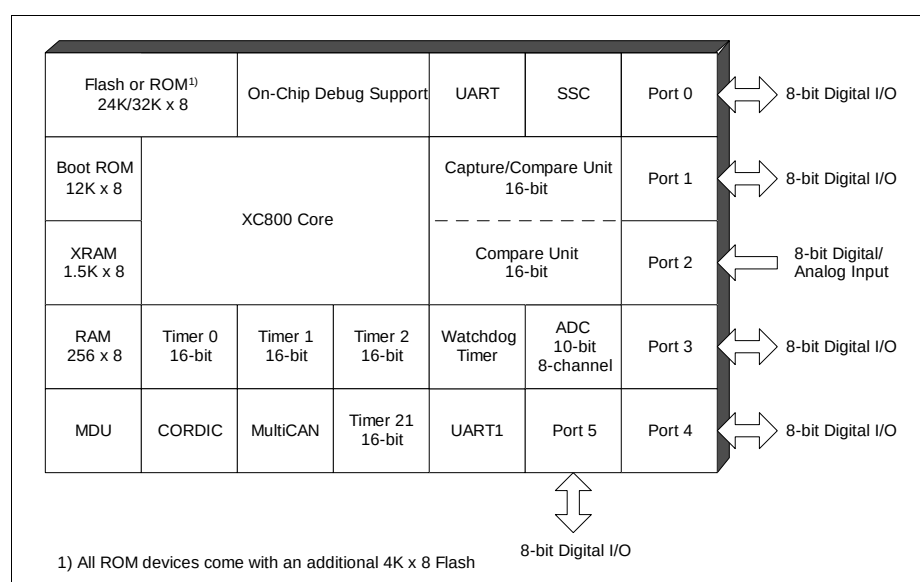
Figure 1 XC886/888 Functional Units
