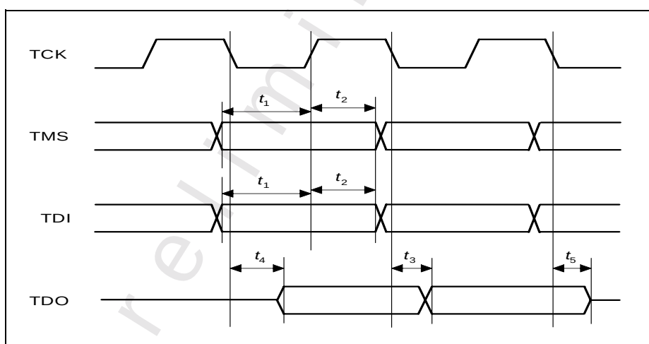
Figure 45 JTAG Timing
