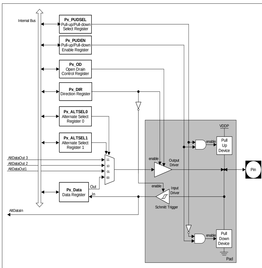
Figure 20 General Structure of Bidirectional Port
