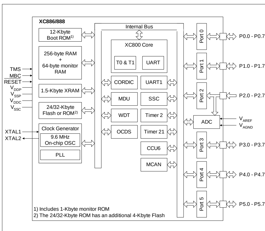
Figure 2 XC886/888 Block Diagram
