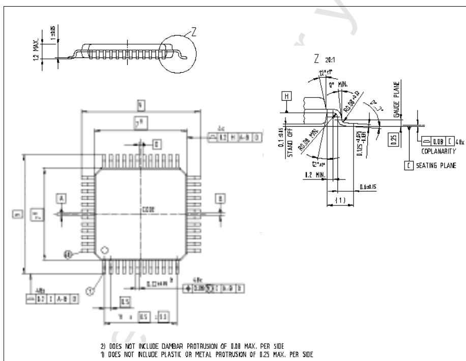
Figure 47 PG-TQFP-48-4 Package Outline
