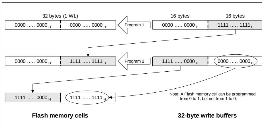
Figure 12 D-Flash Programming
