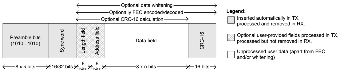
Figure 51: Packet Format
