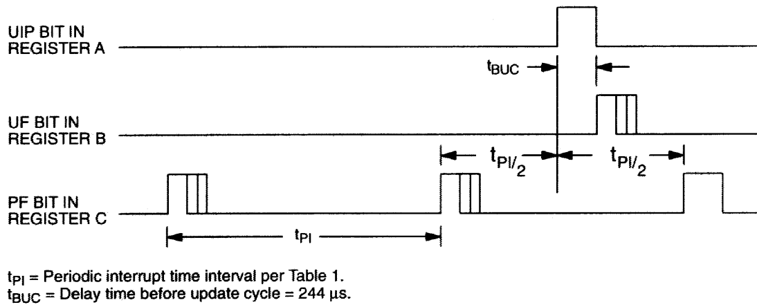
Figure 4. Update-Ended and Periodic Interrupt Relationship
