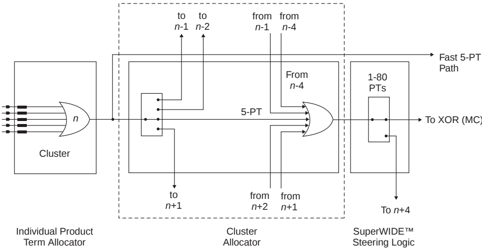
Figure 4. Macrocell Slice
