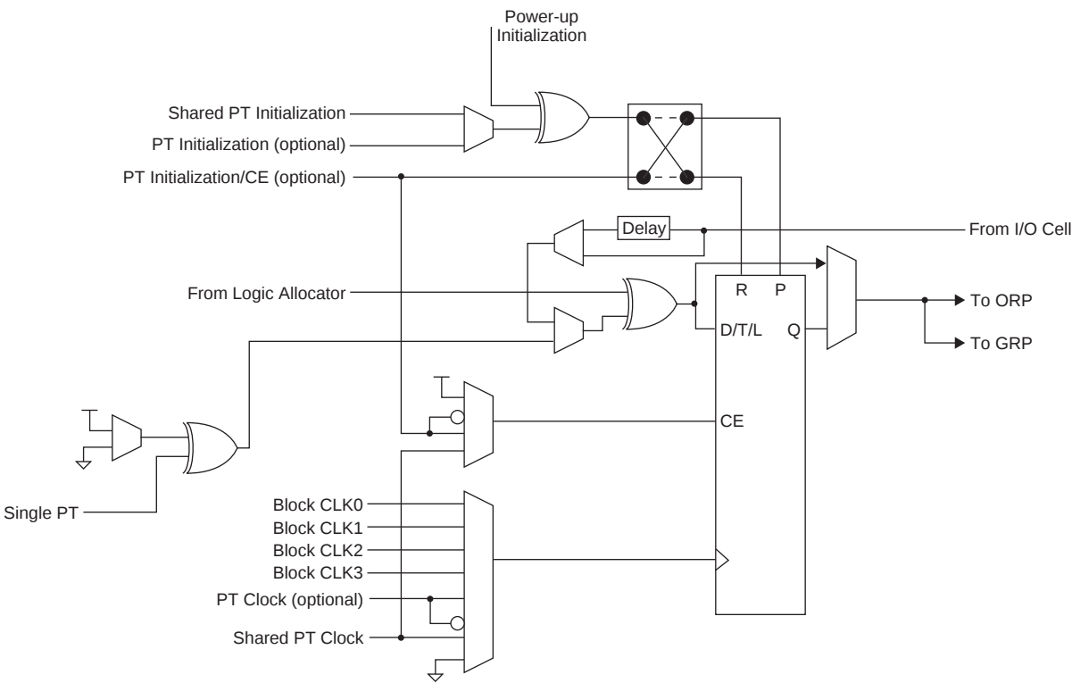
Figure 5. Macrocell
