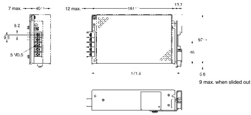
S82J-050□□□D (50 W)
