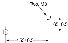
Side Mounting
