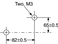
Bottom Mounting
