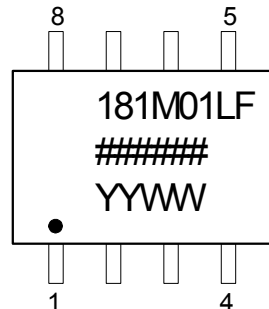
Marking Diagram (ICS181MI-01LF)
