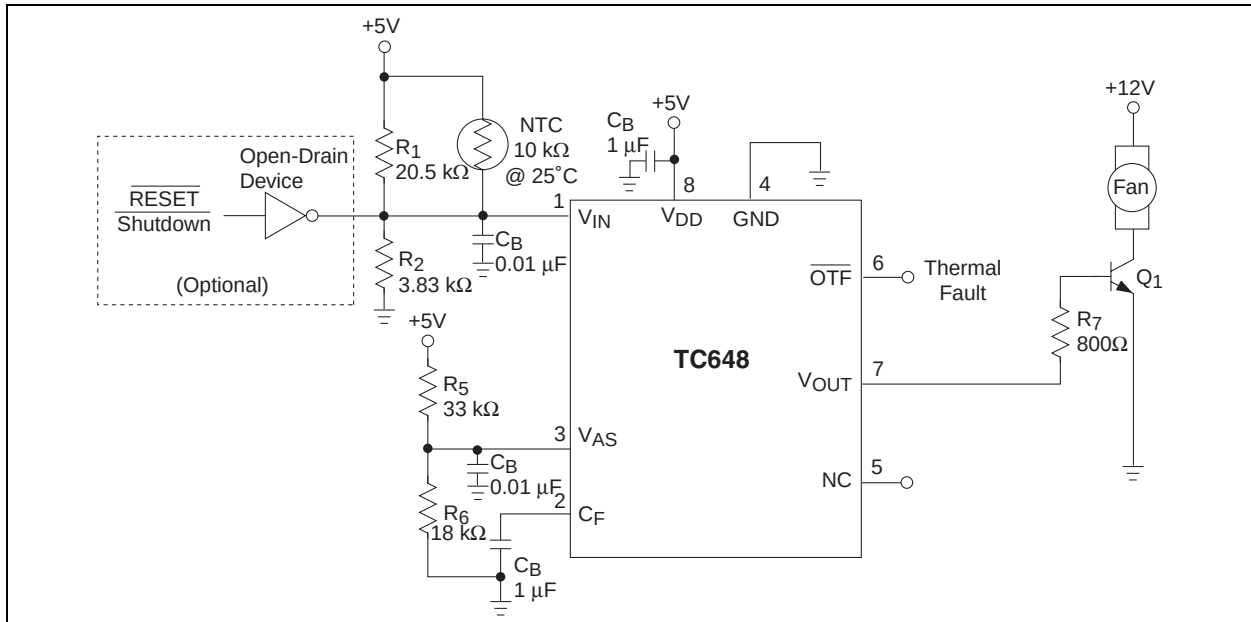
FIGURE 5-8: Design Example.
