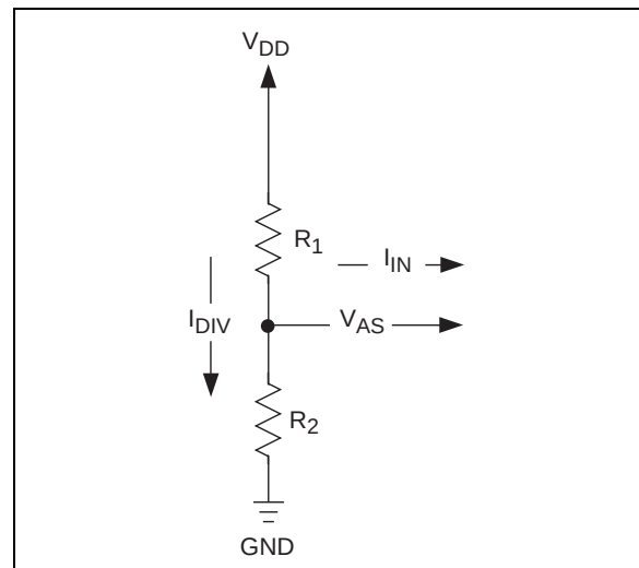
FIGURE 5-5: V_{AS} Circuit.
