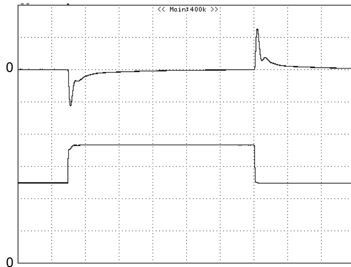
Figure 9: Output voltage response to step-change in load current (75%-50%-75% of I_{o, \text{max}} ; di/dt = 2.5\text{A}/\mu\text{s} ). Load cap: 470\mu\text{F} , 35\text{m}\Omega ESR solid electrolytic capacitor and 1\mu\text{F} ceramic capacitor. Top Trace: V_{\text{out}} (50mV/div, 200 \mu\text{s} /div), Bottom Trace: I_{\text{out}} (5A/div). Scope measurement should be made using a BNC cable (length shorter than 20 inches). Position the load between 51 mm to 76 mm (2 inches to 3 inches) from the module
