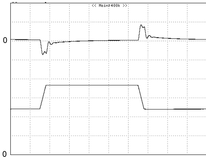
Figure 8: Output voltage response to step-change in load current (75%-50%-75% of I_{o, \text{max}} ; di/dt = 0.1\text{A}/\mu\text{s} ). Load cap: 10\mu\text{F} tantalum capacitor and 1\mu\text{F} ceramic capacitor. Top Trace: V_{\text{out}} (50mV/div, 200 \mu\text{s} /div), Bottom Trace: I_{\text{out}} (5A/div). Scope measurement should be made using a BNC cable (length shorter than 20 inches). Position the load between 51 mm to 76 mm (2 inches to 3 inches) from the module
