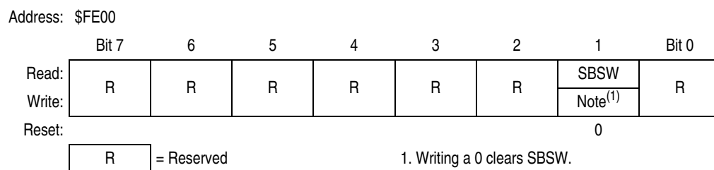
Figure 16-8. Break Status Register (BSR)
