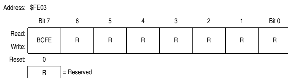
Figure 16-9. Break Flag Control Register (BFCR)
