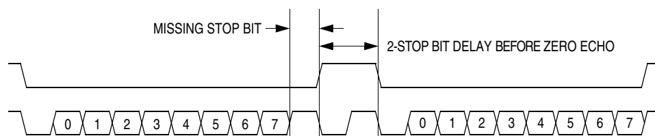
Figure 16-15. Break Transaction
