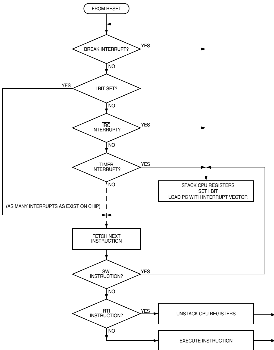
Figure 14-8. Interrupt Processing
