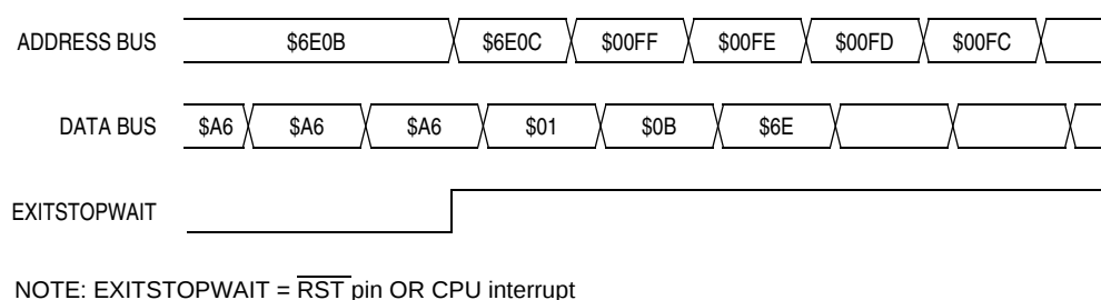
Figure 14-16. Wait Recovery from Interrupt
