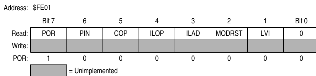
Figure 14-20. SIM Reset Status Register (SRSR)
