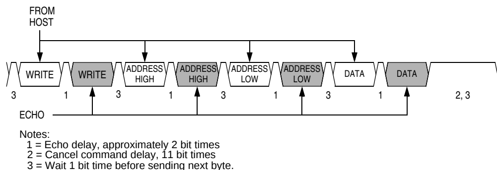
Figure 16-17. Write Transaction
