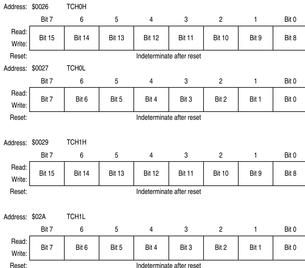
Figure 15-10. TIM Channel Registers (TCH0H/L:TCH1H/L)
