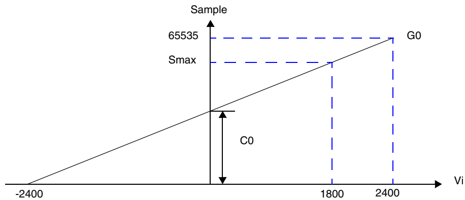
Figure 35. Offset Calculations
