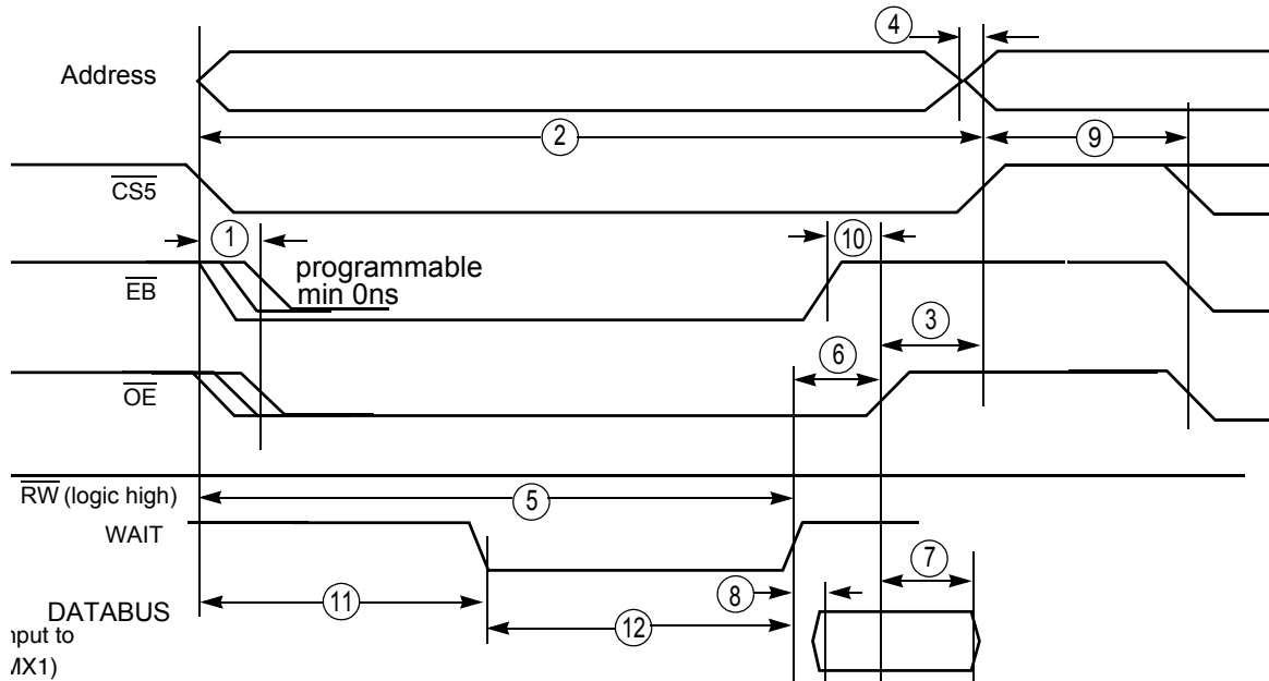
Figure 7. DTACK WAIT Read Cycle DMA Enabled
