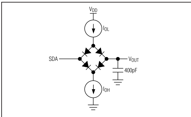
Figure 3. Load Circuit
