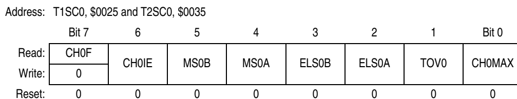
Figure 6-9. TIM Channel 0 Status and Control Register (TSC0)
