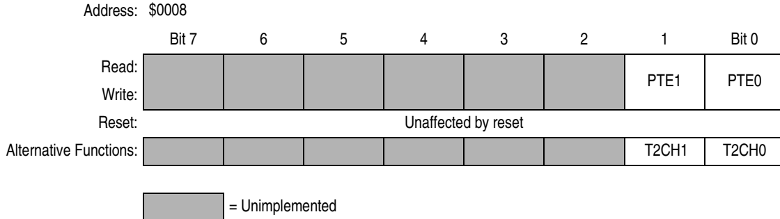
Figure 10-14. Port E Data Register (PTE)
