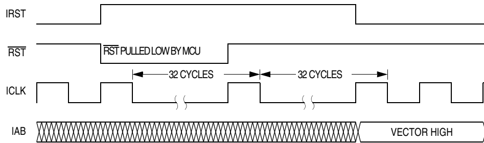
Figure 4-5. Internal Reset Timing
