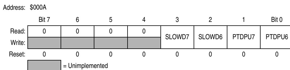
Figure 10-13. Port D Control Register (PDCR)
