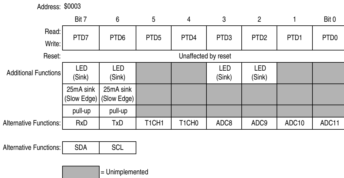
Figure 10-10. Port D Data Register (PTD)
