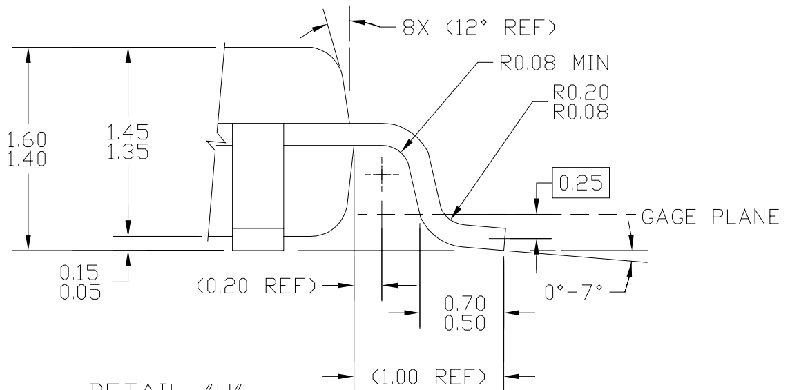
DETAIL "H"
