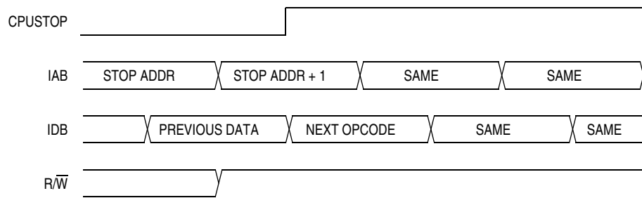
Figure 4-18. Stop Mode Entry Timing
