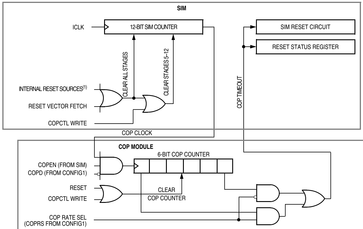
Figure 13-1. COP Block Diagram
