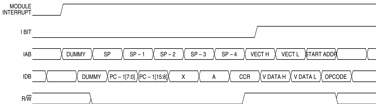
Figure 4-9. Interrupt Entry
