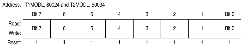
Figure 6-8. TIM Counter Modulo Register Low (TMDL)
