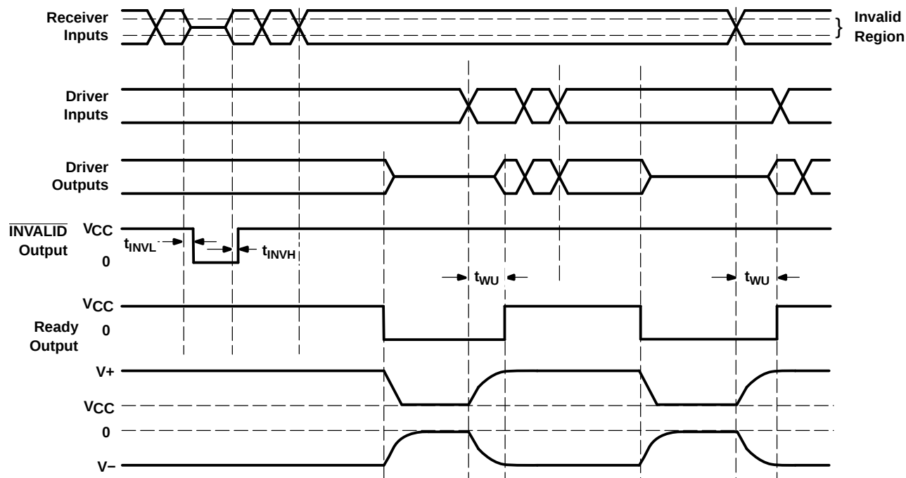
VOLTAGE WAVEFORMS
