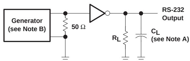
TEST CIRCUIT
