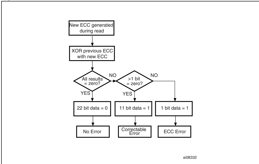
Figure 23. Error detection
