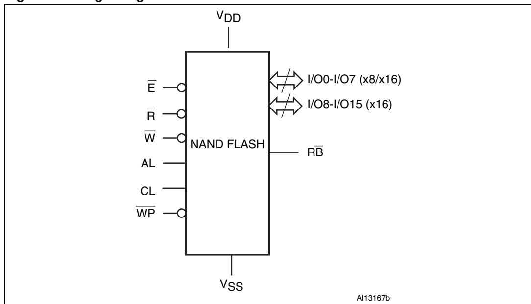
Figure 2. Logic diagram
