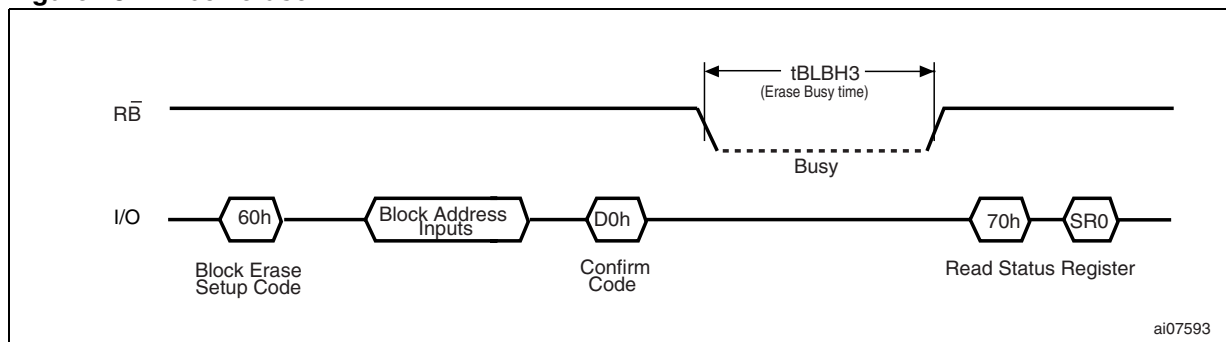
Figure 18. Block erase
