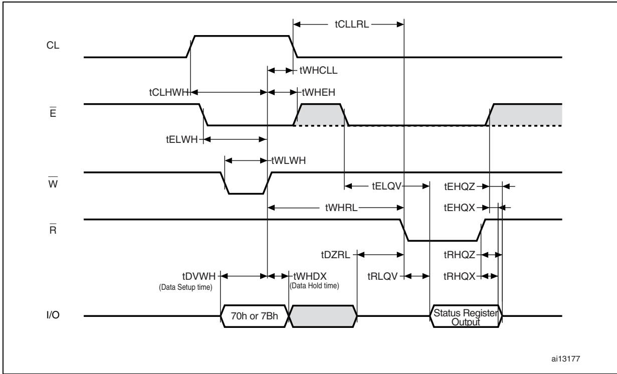
Figure 31. Read status enhanced waveform
