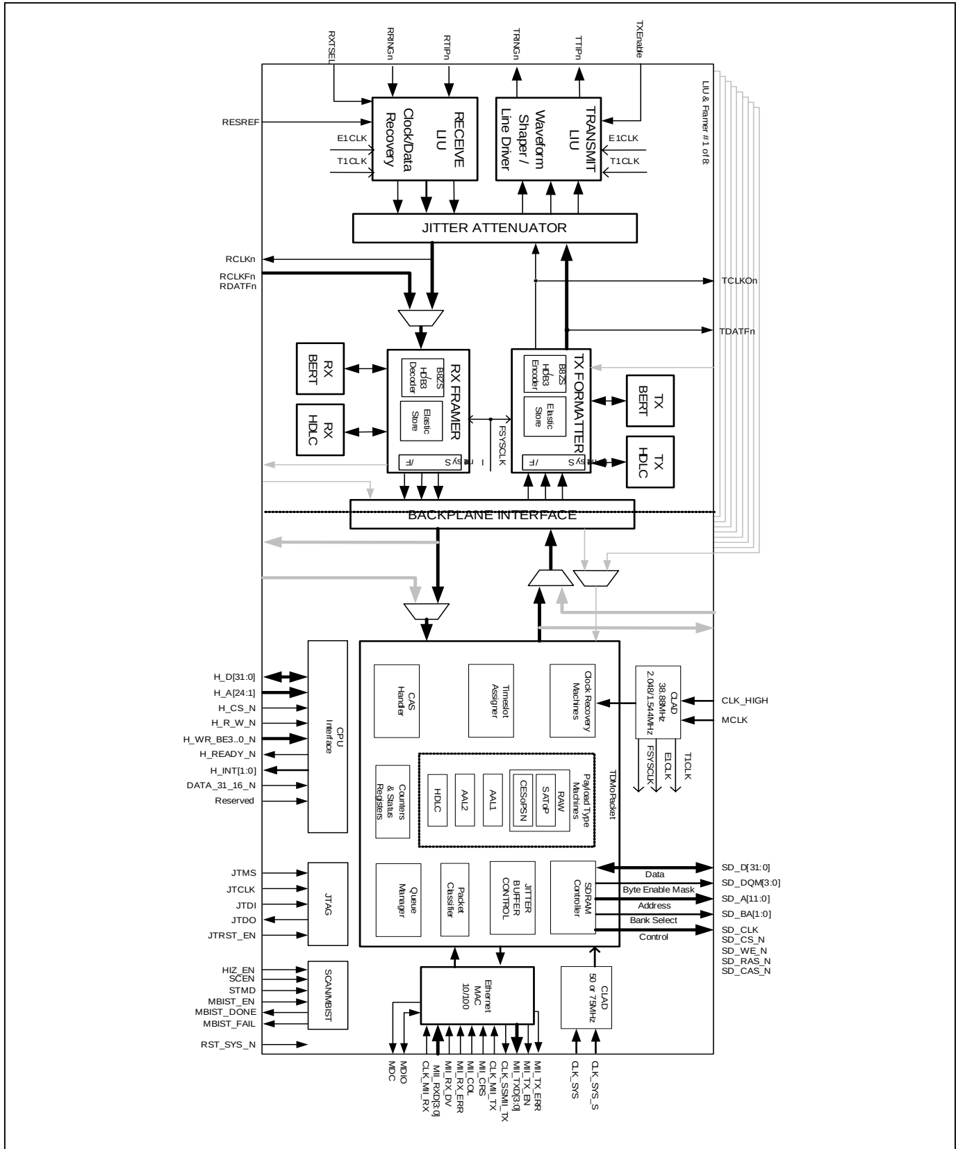
Figure 8-1. Internal Mode
