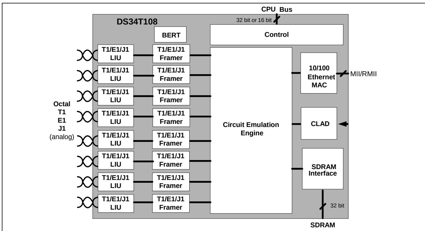
Figure 1-1. Block Diagram
