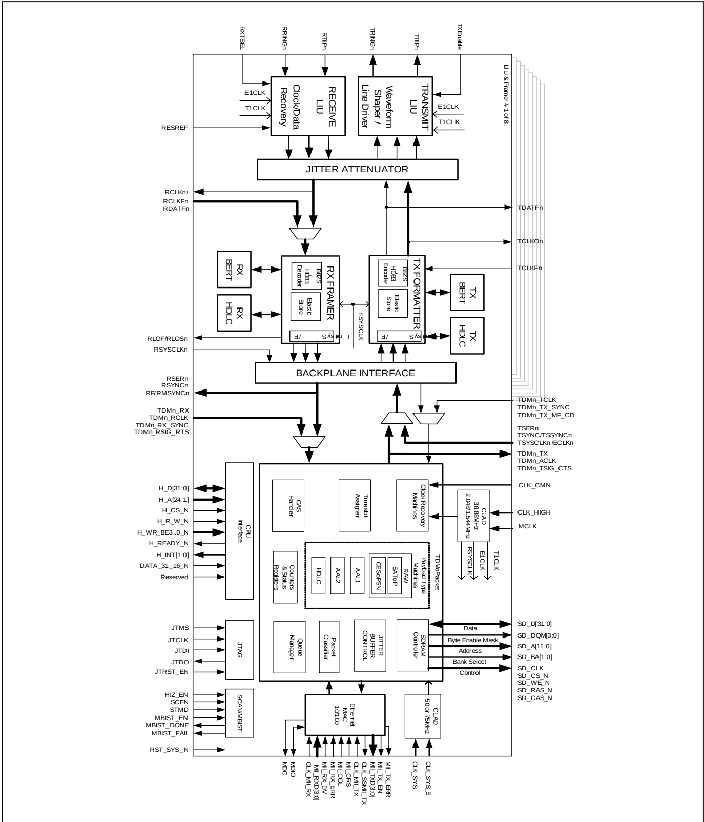
Figure 6-1. DS34T108 Functional Block Diagram
