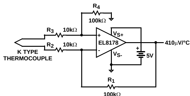
FIGURE 29. THERMOCOUPLE AMPLIFIER
