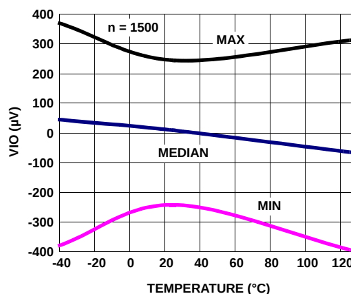
FIGURE 16. V_{OS} vs TEMPERATURE, V_S = \pm 2.5V
