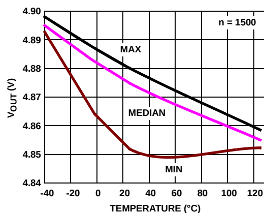
FIGURE 22. V_{OUT} HIGH vs TEMPERATURE, V_S = \pm 2.5V , R_L = 1k
