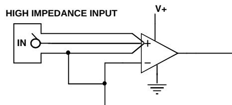
FIGURE 27. GUARD RING EXAMPLE FOR UNITY GAIN AMPLIFIER
