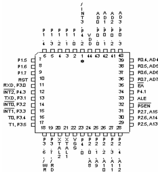
44-Pin PLCC
