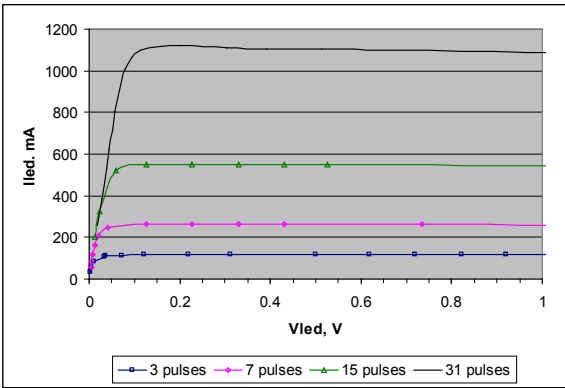
Load regulation at V_{CC} = 5.5V @ 25^{\circ}C
