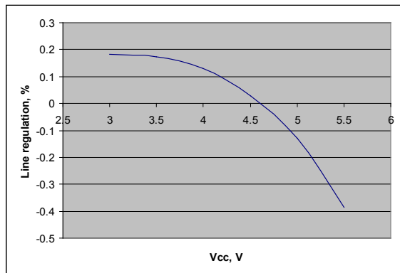
Line regulation at V_{LED} = 100\text{mA}
