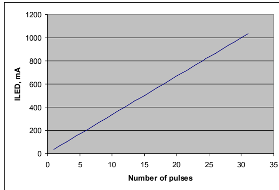
DAC linearity at V_{LED} = 500\text{mV}
