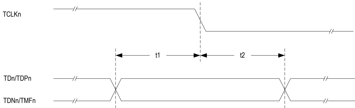
Figure-52 Transmit Clock Timing Diagram
