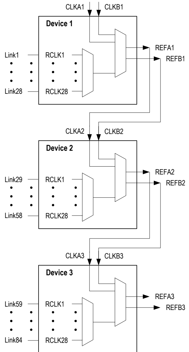
Figure-44 Three IDT82P2828 in Parallel
