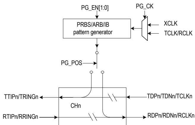
Figure-26 Pattern Generation (1)
