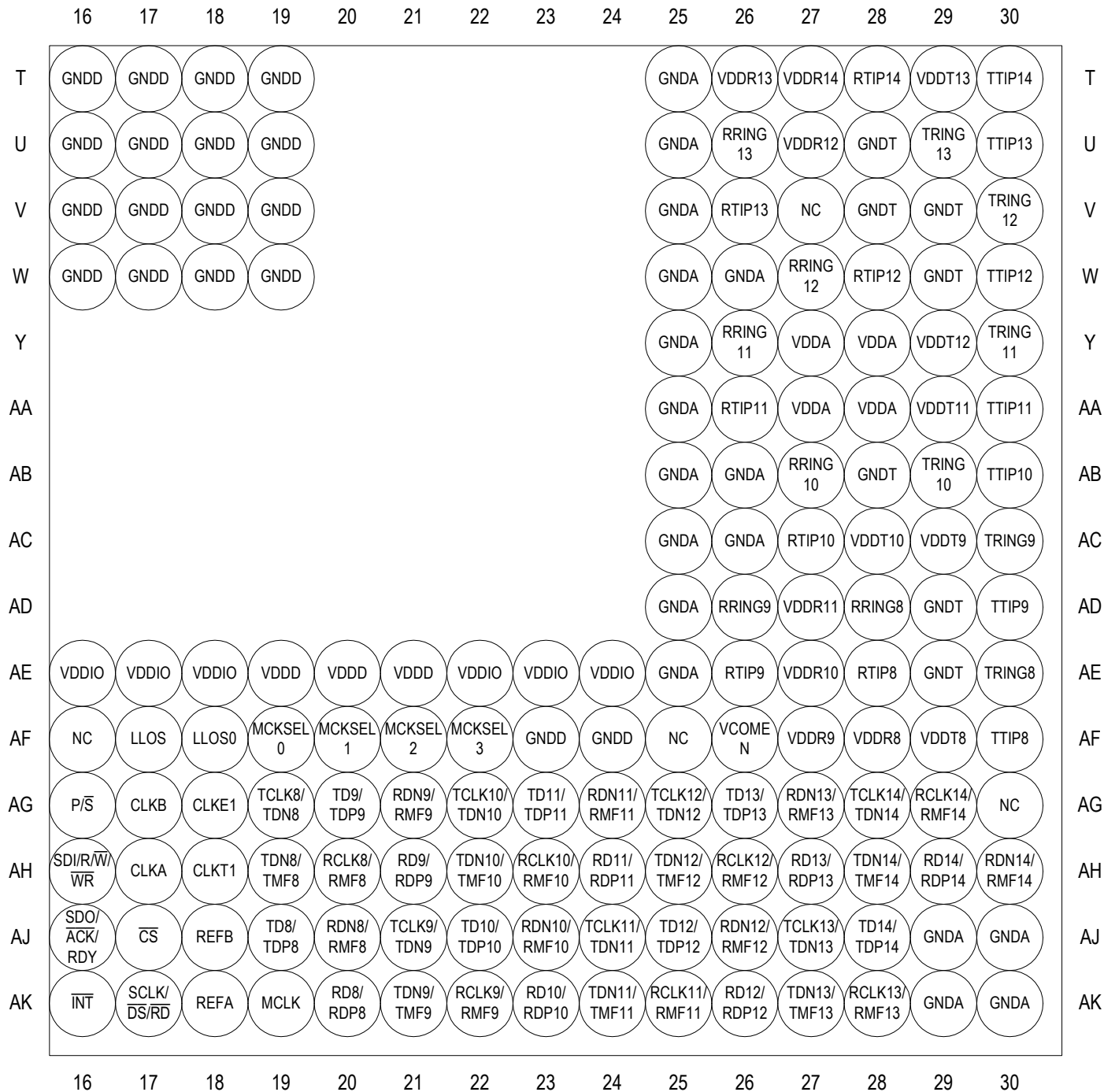
Figure-6 640-Pin PBGA (Top View) - Bottom Right
