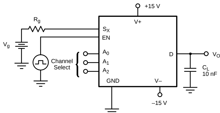
FIGURE 5. Charge Injection
