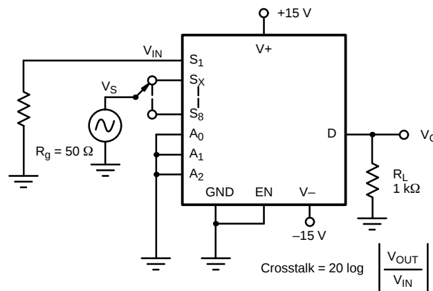
FIGURE 7. Crosstalk
