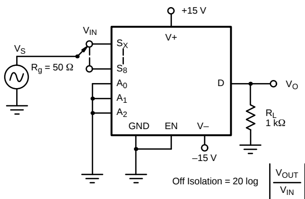
FIGURE 6. Off Isolation
