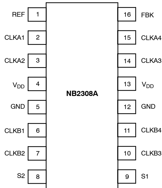
Figure 2. Pin Configuration
