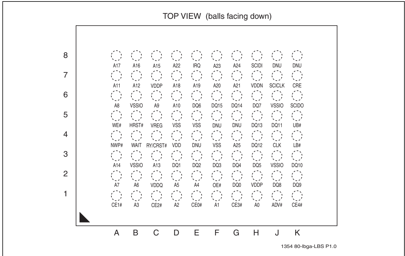
FIGURE 2-1: Pin Assignments for 80-ball LBGA
