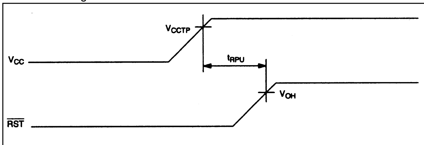
POWER-UP Figure 12
