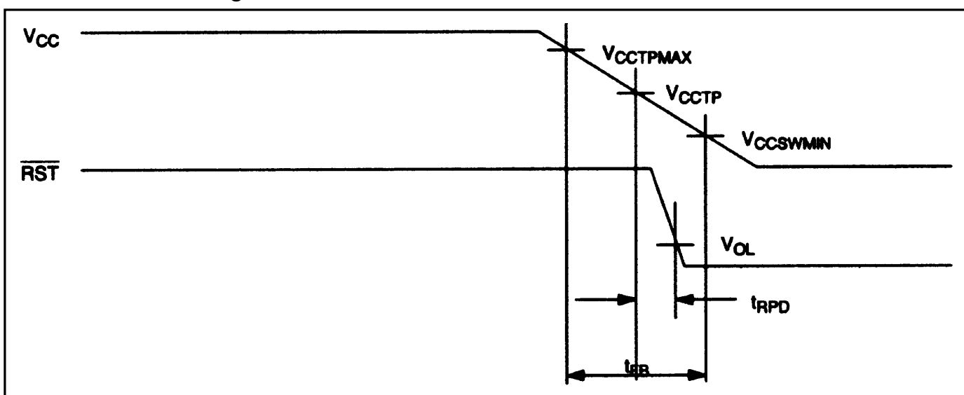
POWER-DOWN Figure 13
