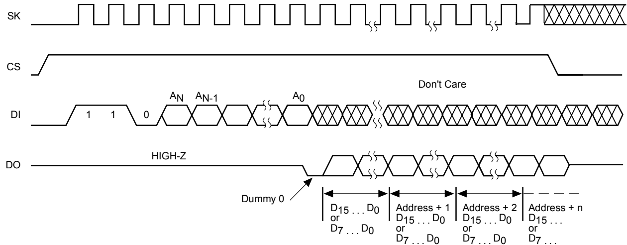
Figure 2. Read Instruction Timing
