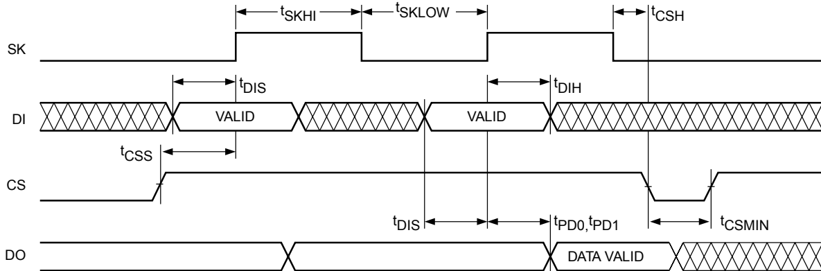
Figure 2. Read Instruction Timing
