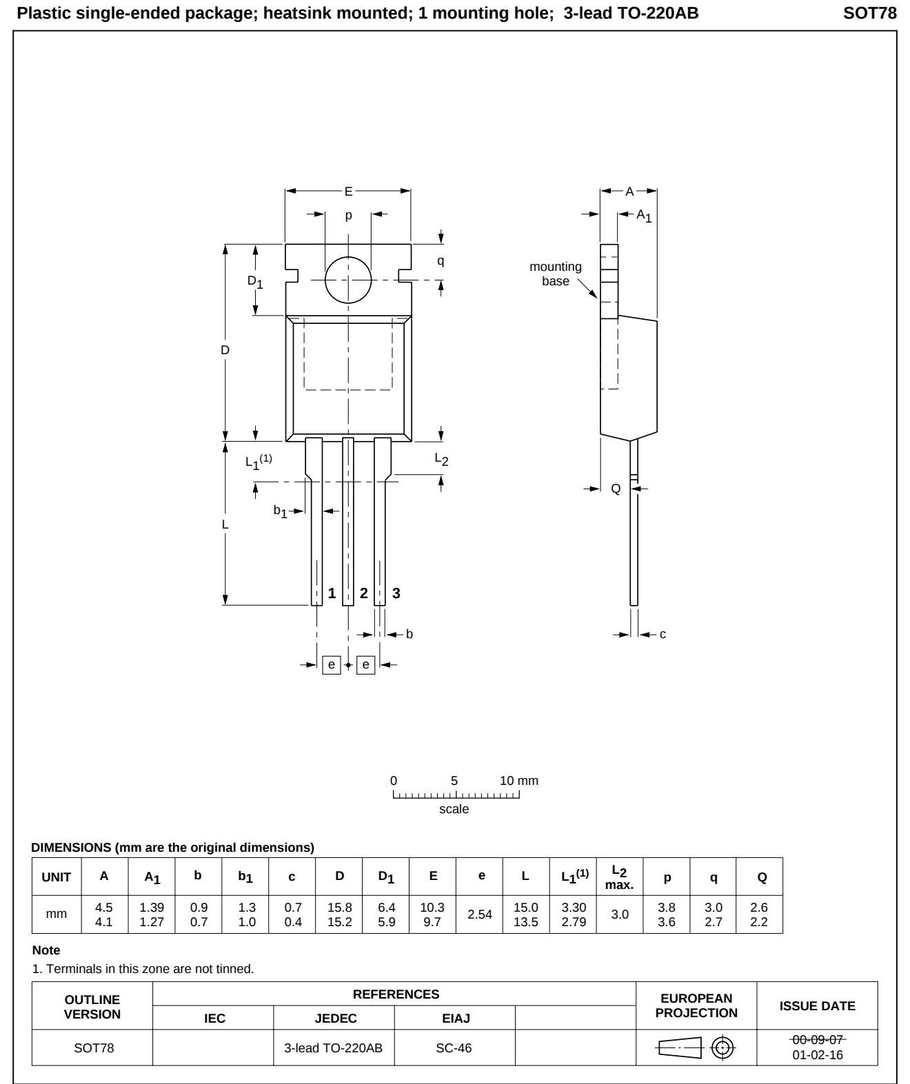
Fig 14. SOT78 (TO-220AB).
