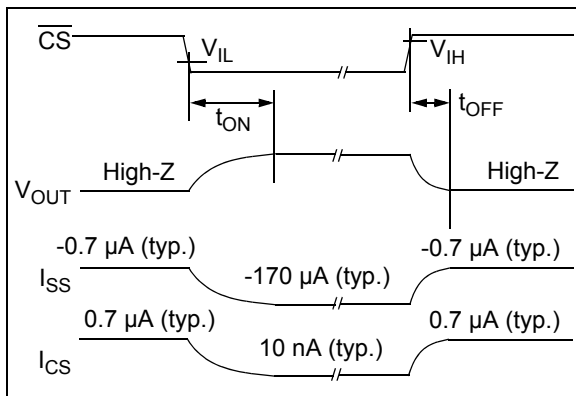
FIGURE 1-1: Timing Diagram for the Chip Select ( \overline{\text{CS}} ) pin on the MCP6273 and MCP6275.
