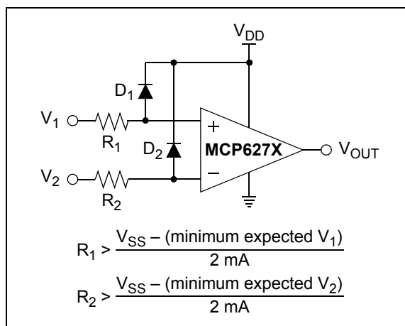
FIGURE 4-2: Protecting the Analog Inputs.
